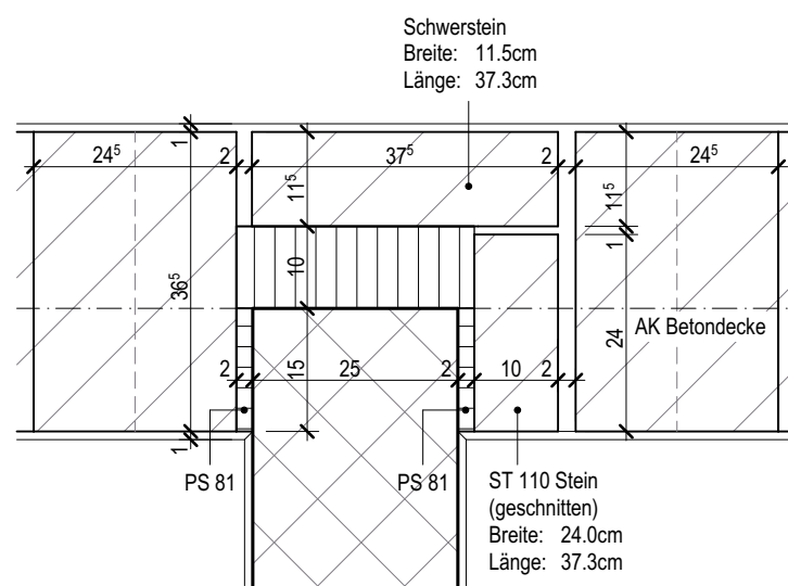
Detail 1.1
