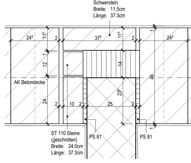
Detail 1.2.2
