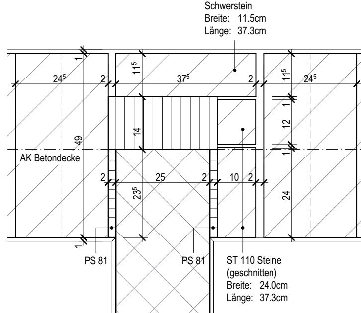
Detail 1.2.1
