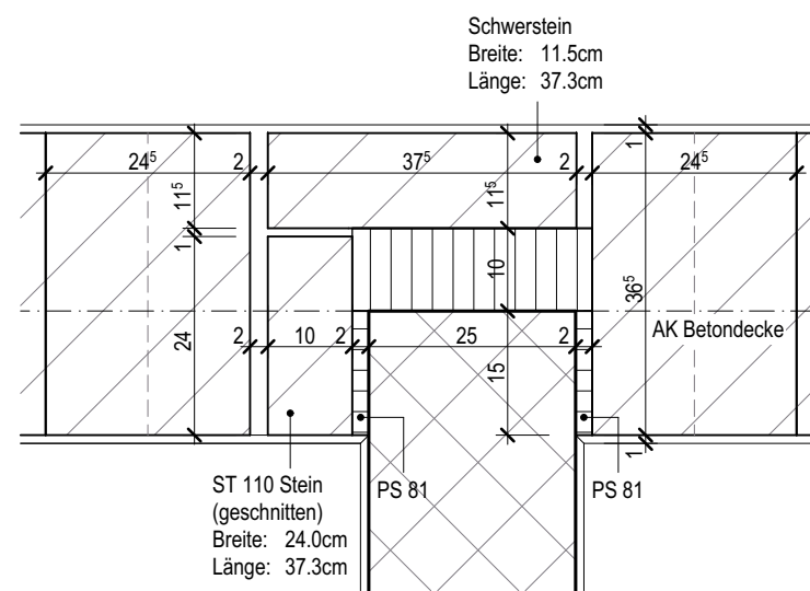
Detail 1.2
